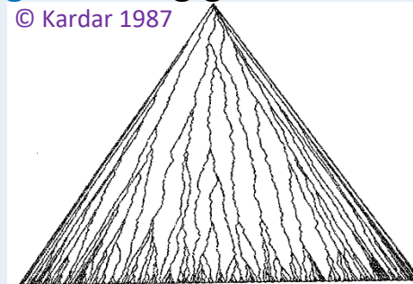
Coalescence of geodesics in D=2 dim.
